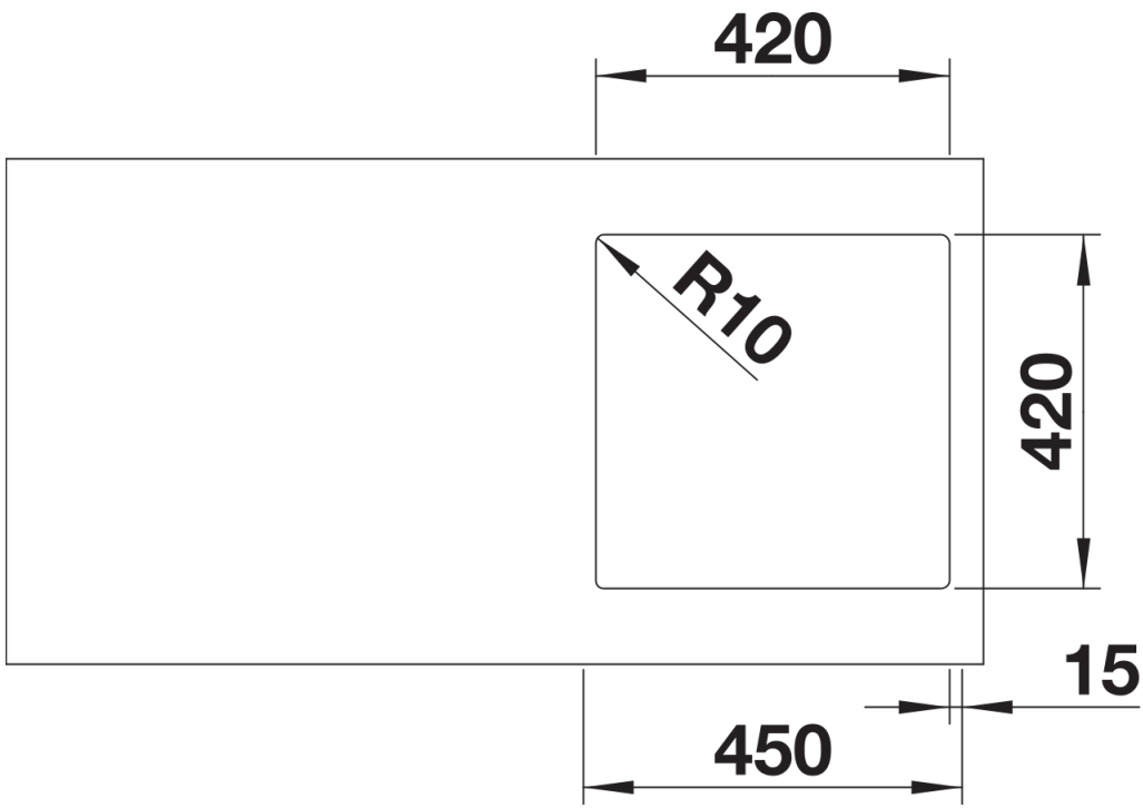
Cut-out
