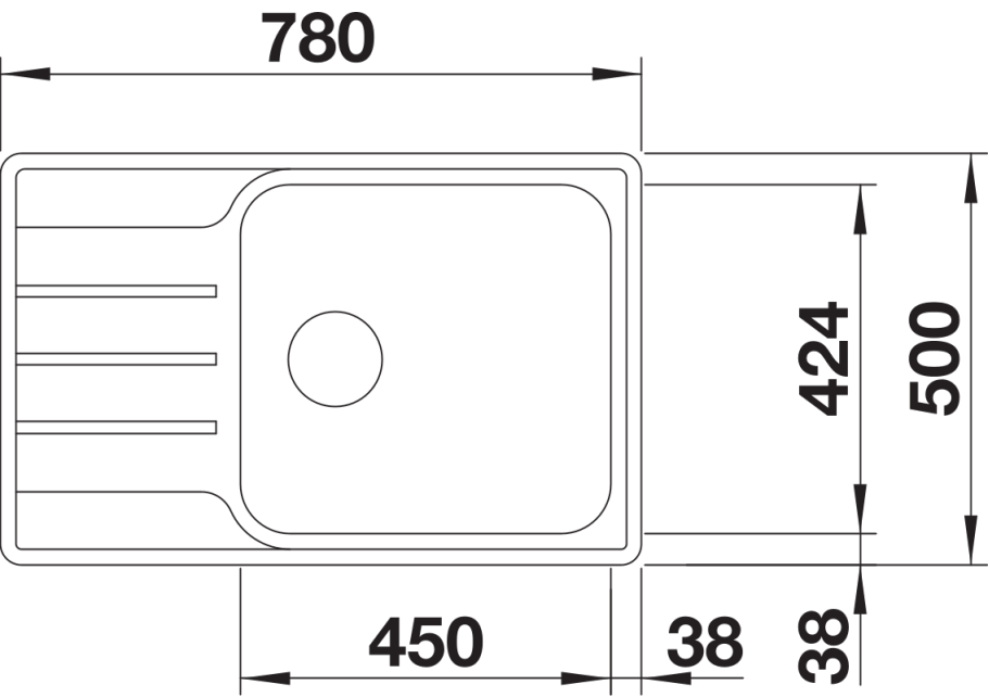
Top view
