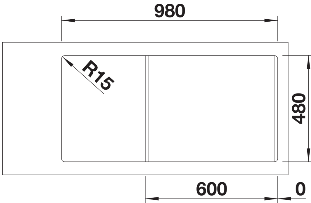
Cut-out
