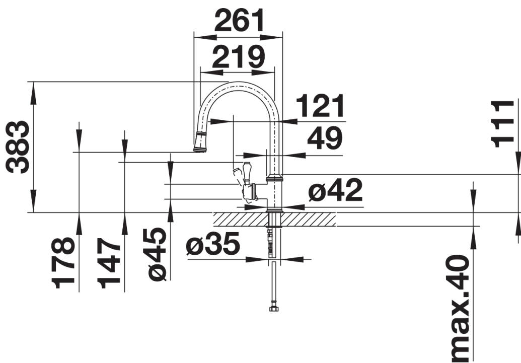
Side view
