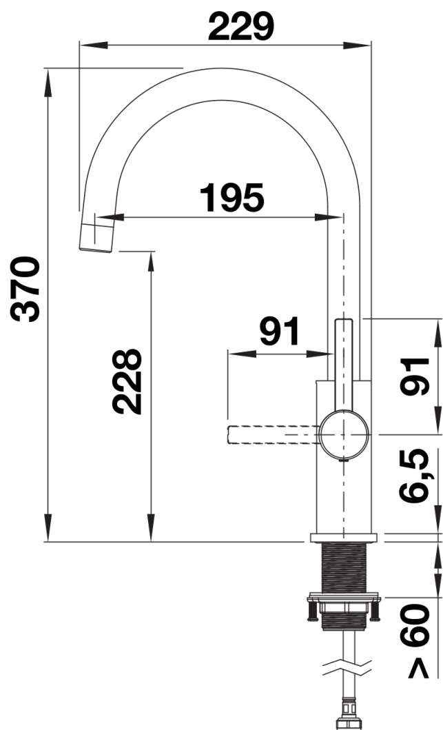
Side view
