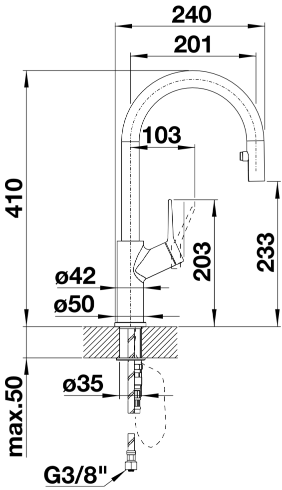
Side view
