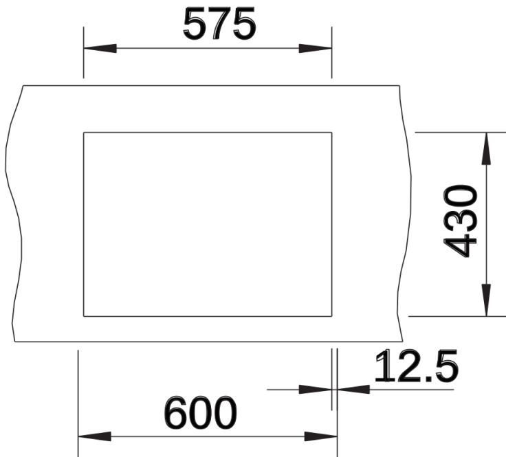
Cut-out
