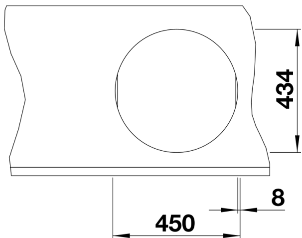
Cut-out
