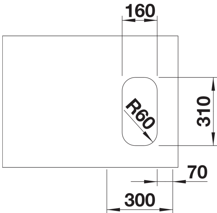
Cut-out
