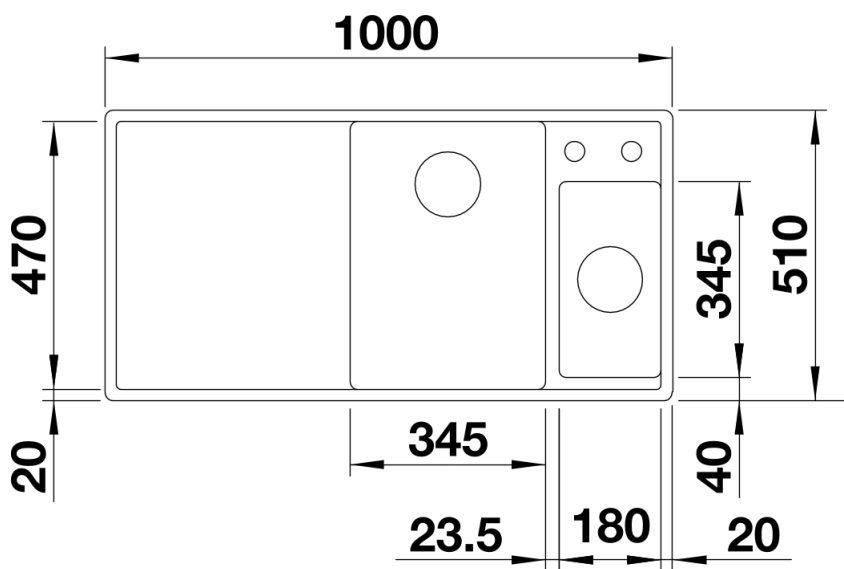
Top view
