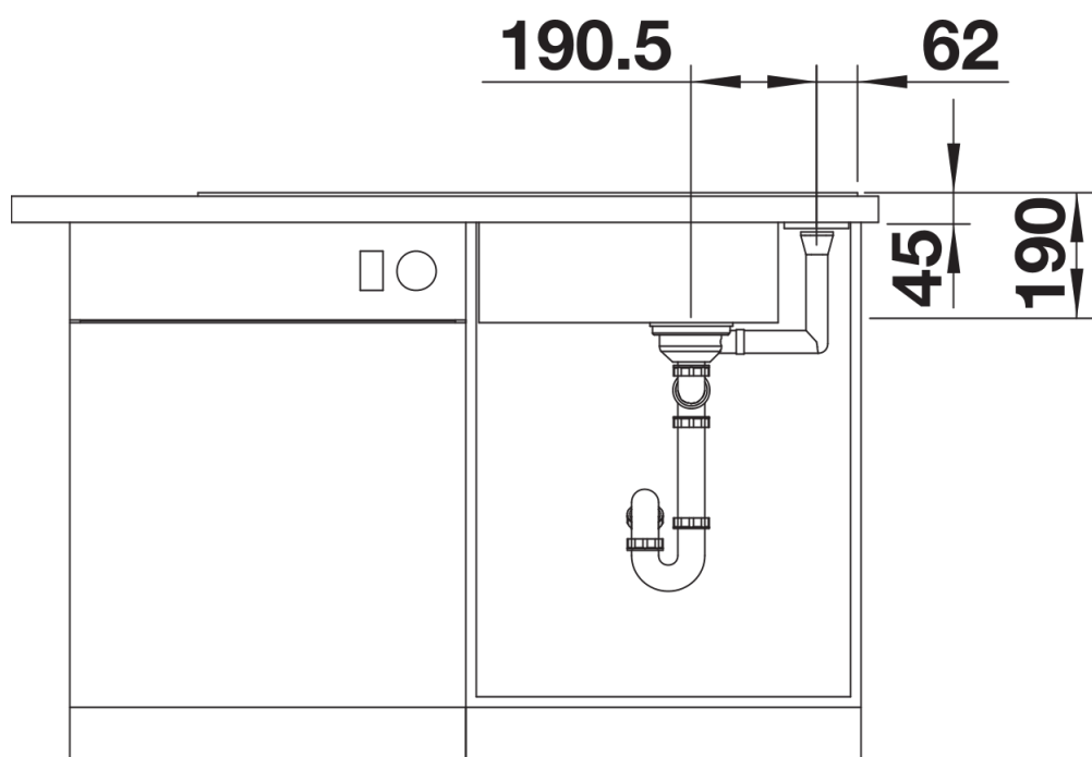
Front view
