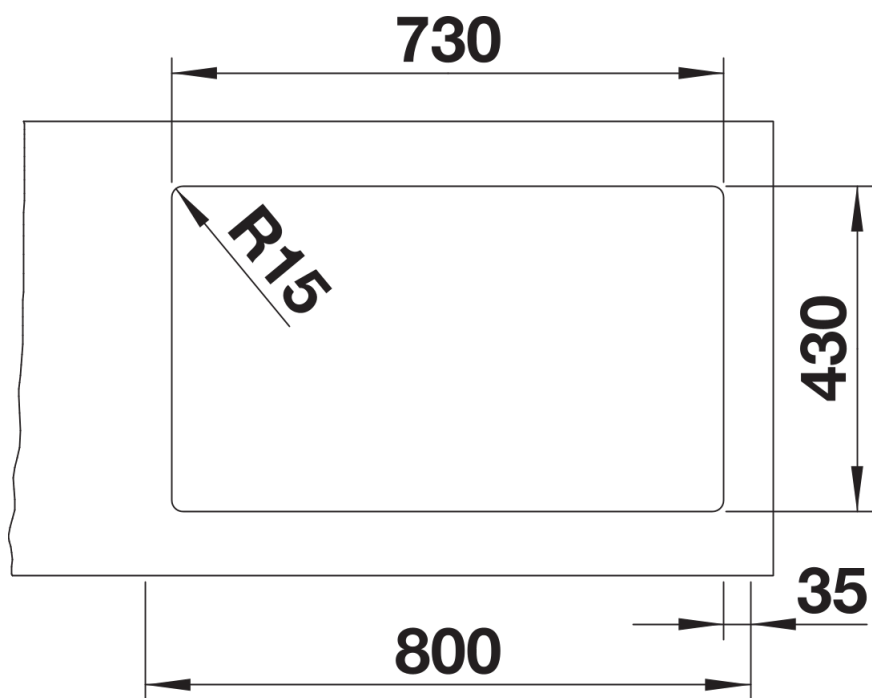
Cut-out
