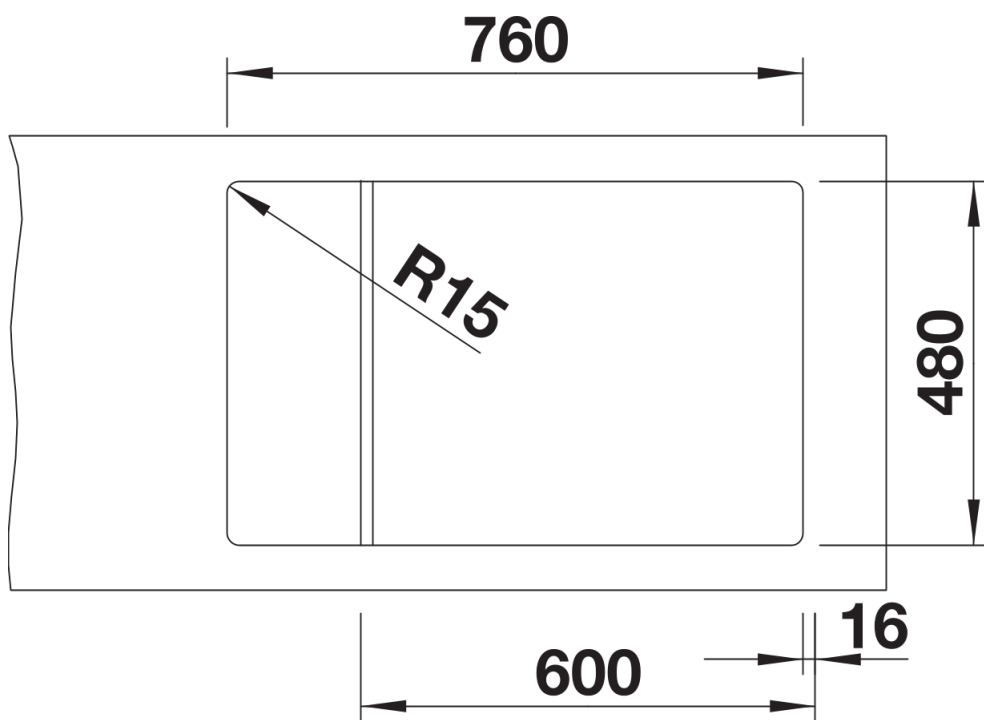
Cut-out
