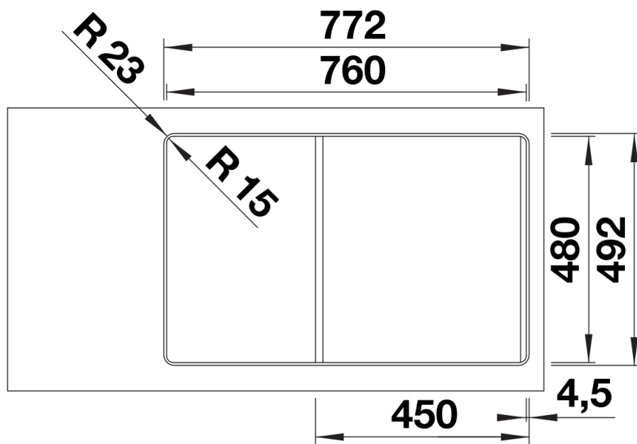
Cut-out
