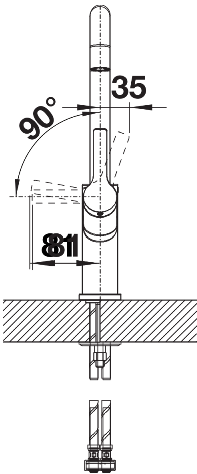
Side view hand gear 2D
