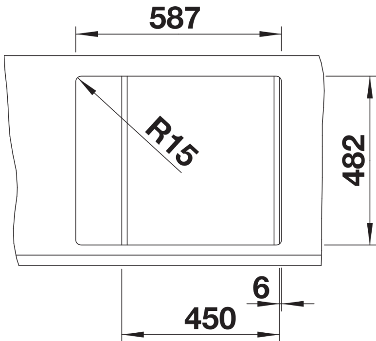
Cut-out
