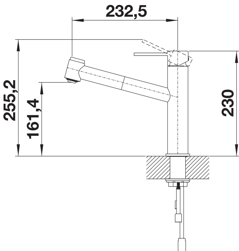
Side view
