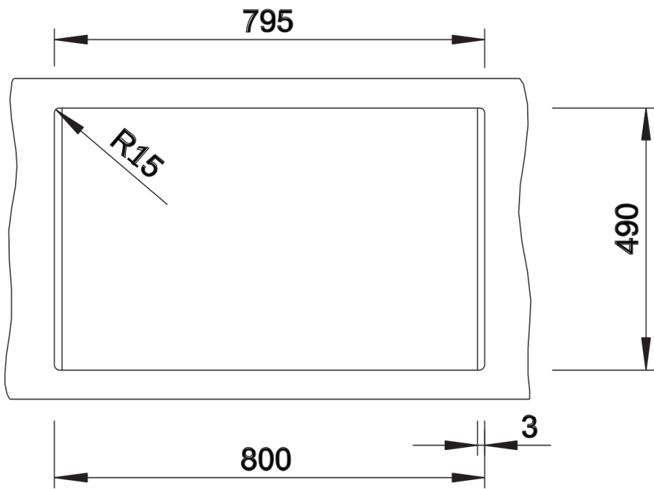
Cut-out
