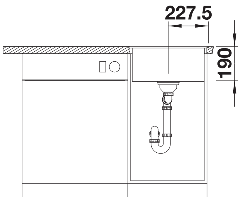
Front view
