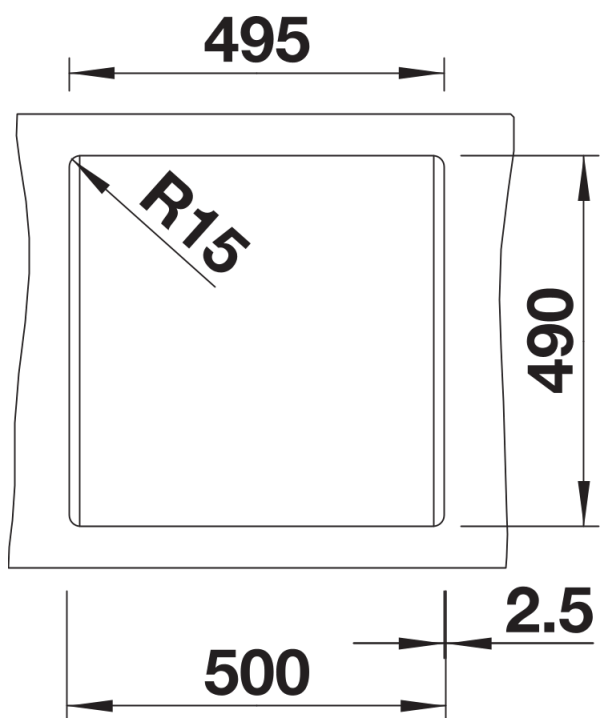
Cut-out
