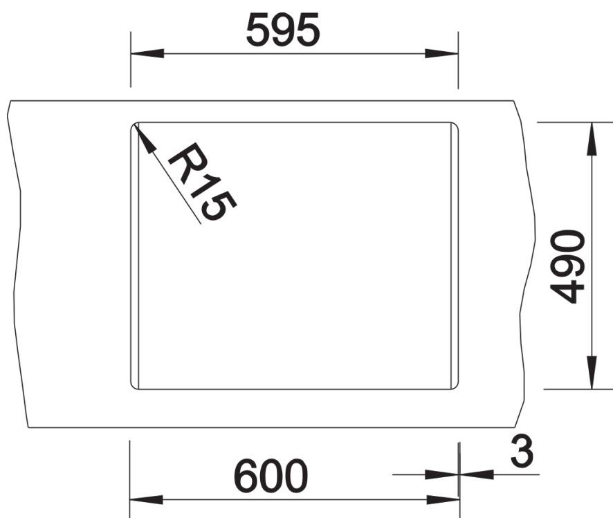
Cut-out
