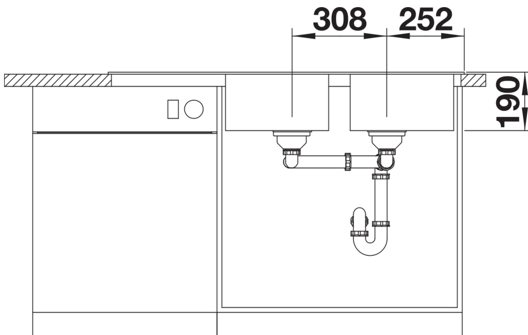
Front view
