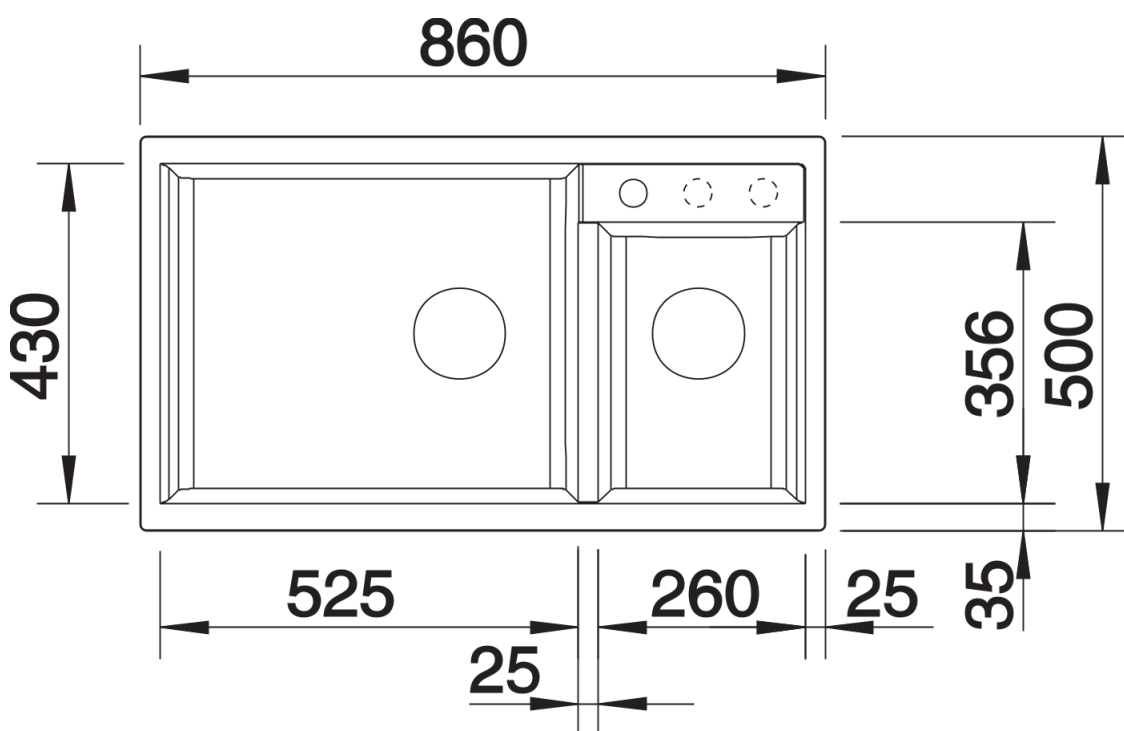
Top view
