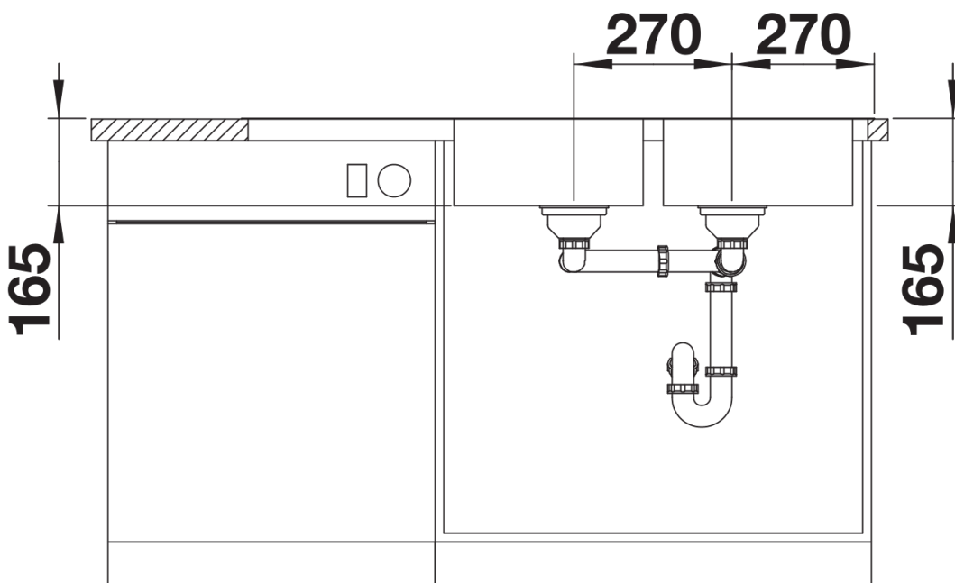
Vista frontal
