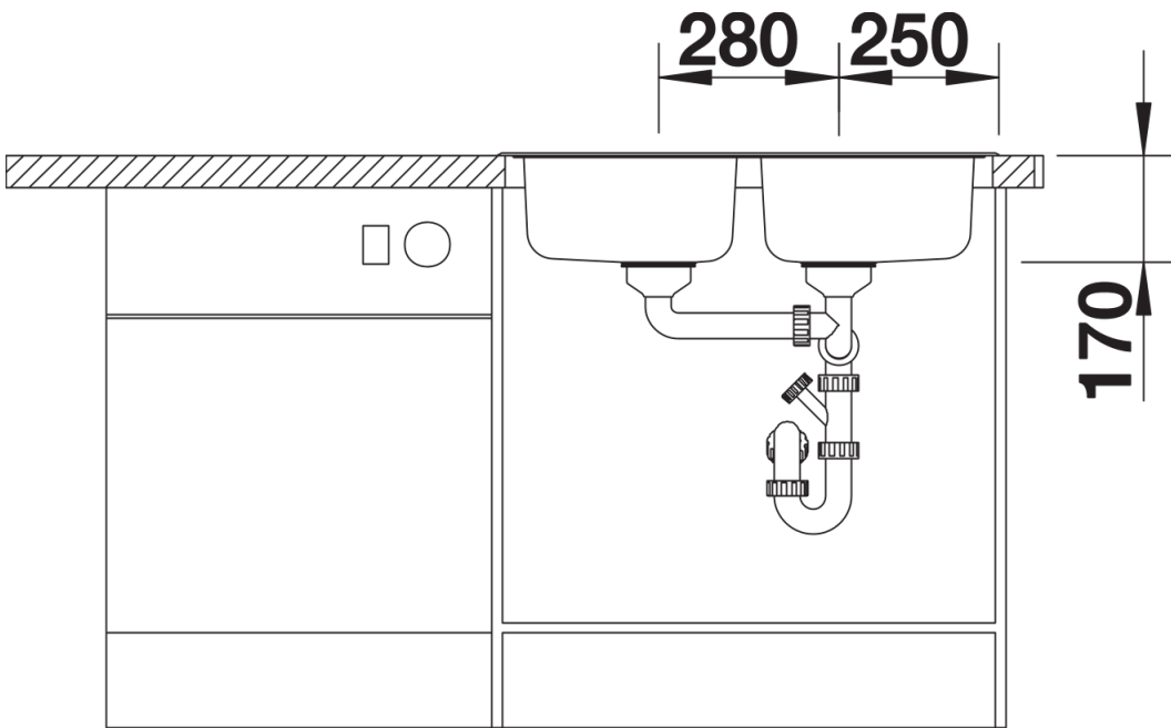
Vista frontal
